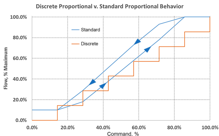
Figure 3: DPV and Continuous Proportional Valve Performance Curves
